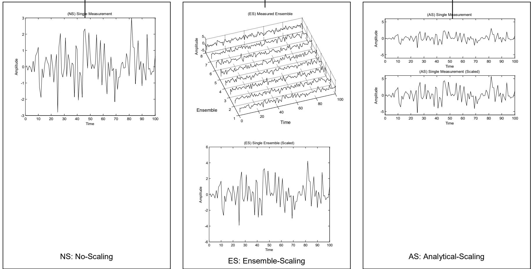
Figure 525.2-1. Basic TWR test modes as related to time trace scaling.
